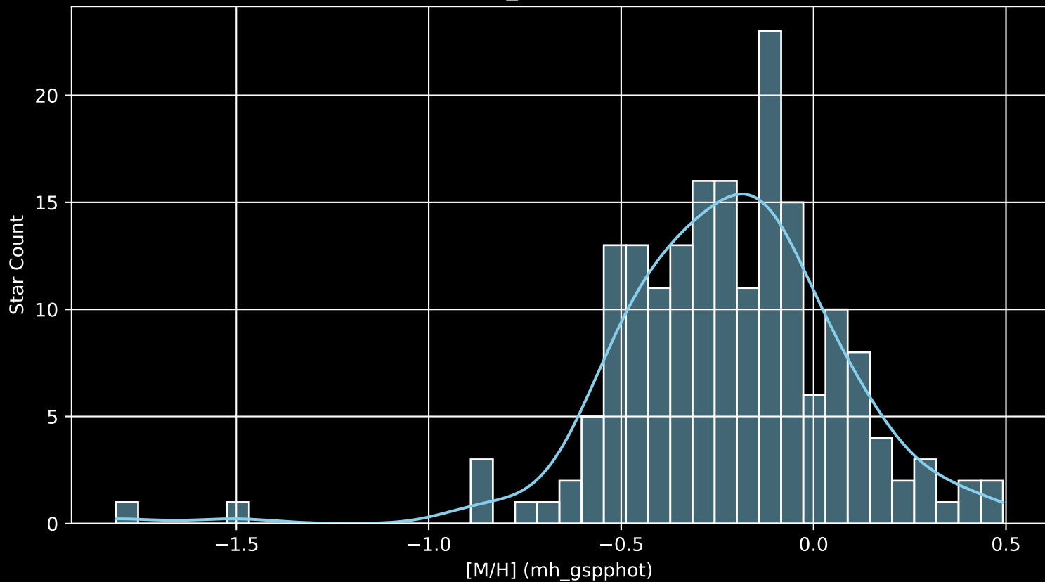
APOGEE DR17 Field: [232+38_MGA [M/H] (mh_gspphot) (n= 183)
