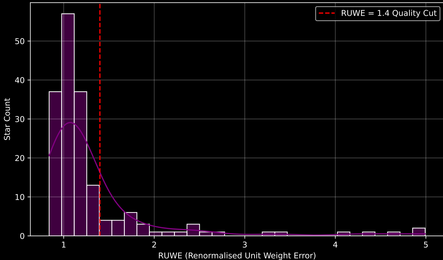
GAPOGEE DR17 Field [232+38_MGA] RUWE Distribution (n= 176)
