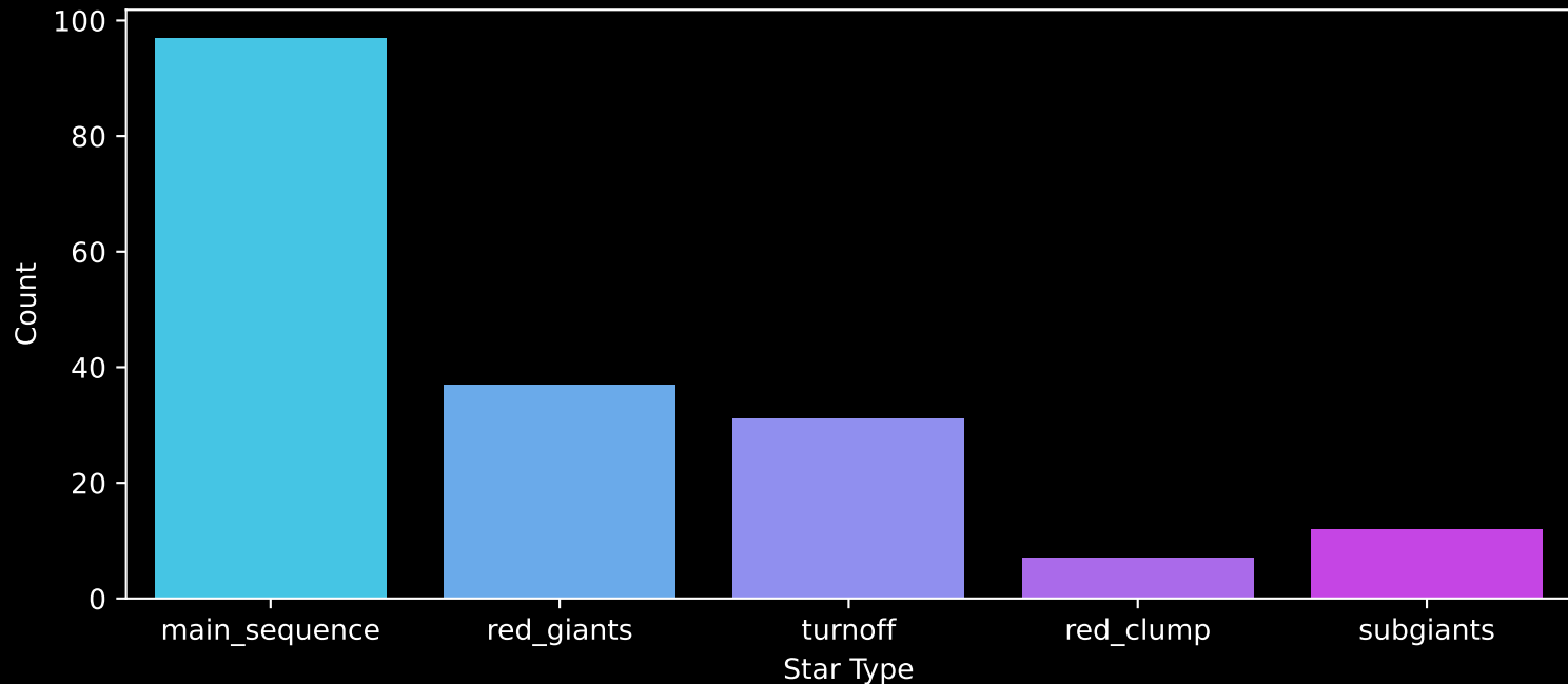
APOGEE DR17 Field: [232+38_MGA] Count plot of Star Type
