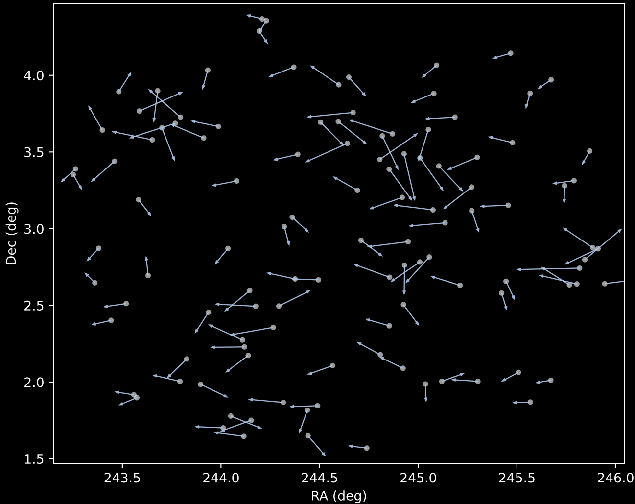
APOGEE DR17 Cluster 1 Proper Motion Vectors (n=112)
