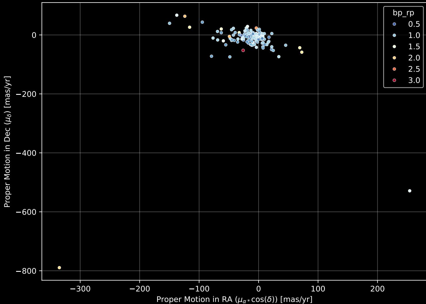
APOGEE DR17 Field: [232+38_MGA] Proper Motion Diagram (n= 184)
