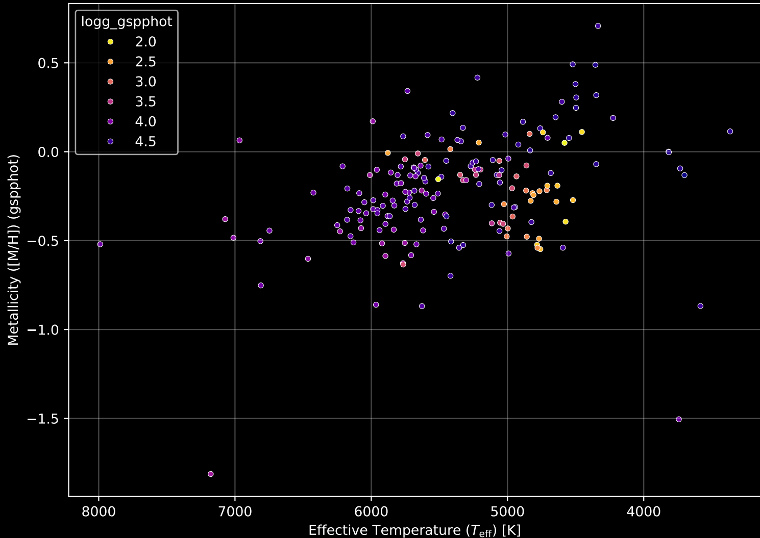
APOGEE DR17 Field: [232+38_MGA] Stellar Population Parameters (n= 184)
