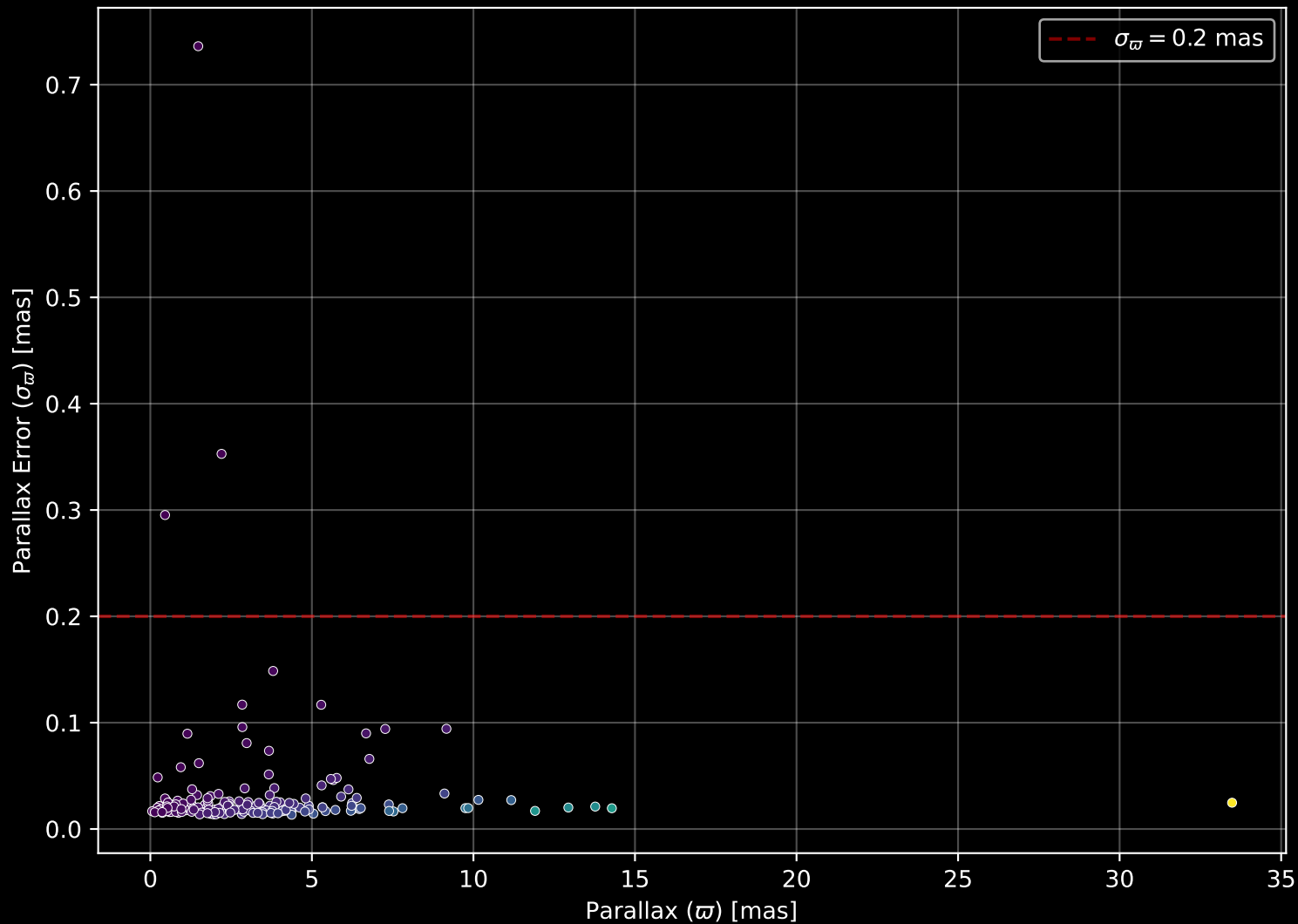
APOGEE DR17 Field: [232+38_MGA] Parallax Quality (n= 184)
